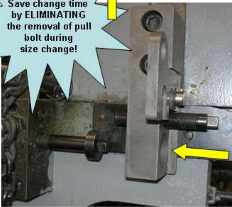
K0.998.495.2 Quick Release Swing Out Shim Plate
